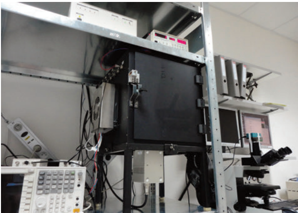
Figure 2b) In the center one can see a lightproof photomultiplier, into which probes are placed for counting emitted photons/sec \times cm 2 .
