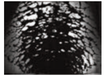
Figure 2. Wrong spraying temperature (only 2 °C lower from optimal), results in too large droplet size, significant problems in chemical recovery and boiler operation.
